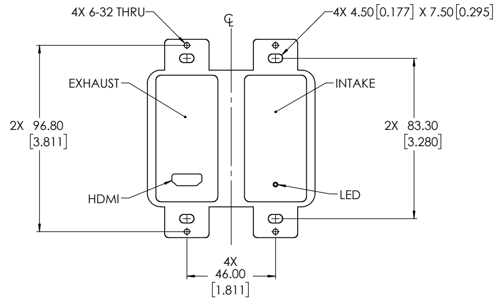
WALLPLATE REMOVED
